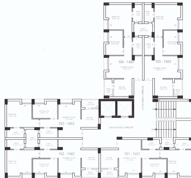
TYPICAL FLOOR PLAN ( 1st to 14th ) BUILDING - C & D
