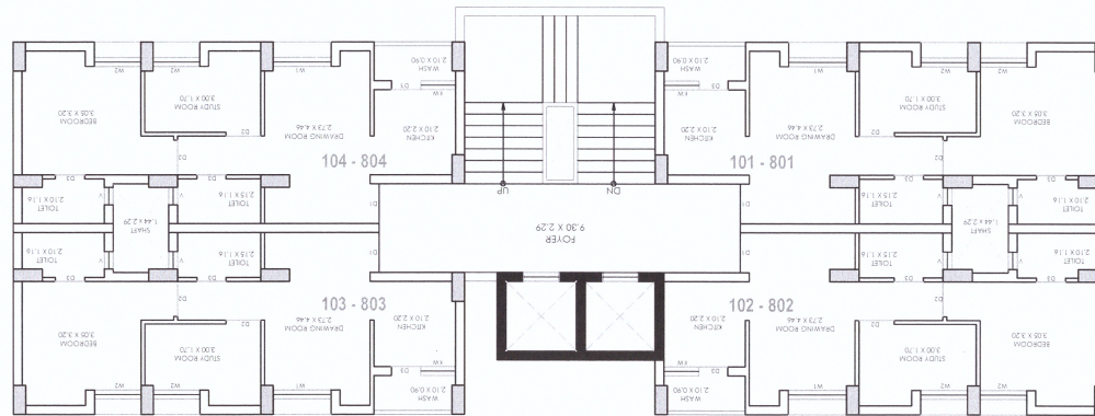
TYPICAL FLOOR PLAN (1st to 8th) BUILDING-A,B,D,E,F,G,H & I
